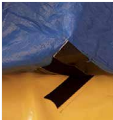
Detail of the fixing between the tank and the liner.
